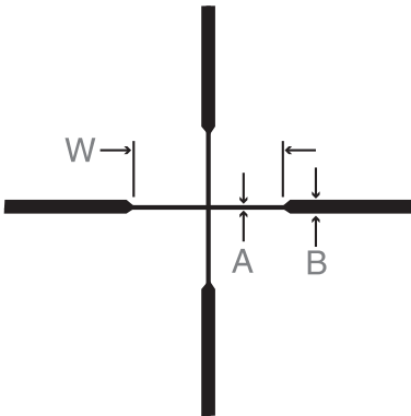
Reticle Subtenions (in mils)
